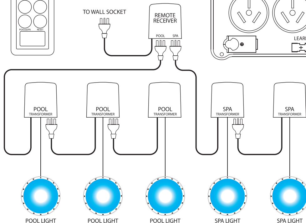
Example Connection Diagram showing multiple light connection
