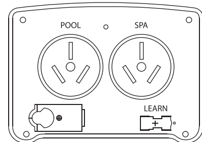
Receiver Base
